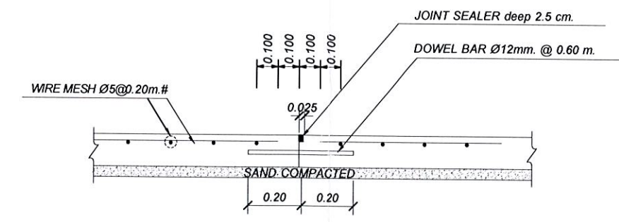
CJ-1 CONTRACTION JOINT DETAIL 1 : 20
