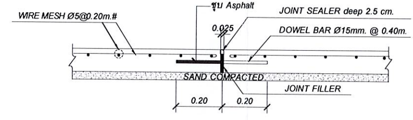
EXJ-1 ; EXPANSION JOINT DETAIL 1 : 20
